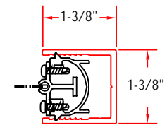
FULLY ASSEMBLED RECESSED SIDE TRACK
